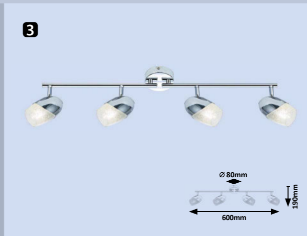
3 5923 M G • LED 4W (400lm, 4000K) incl. E-14/ 4x max. 40W IP20 • 19624 chrome
