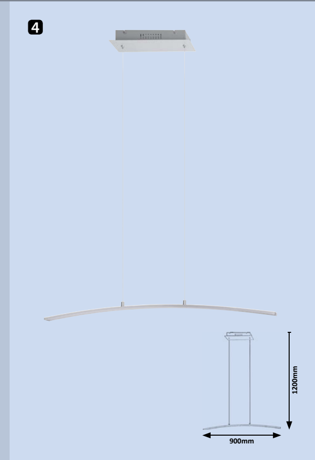
4 5759 (M) (P) • LED / 21W (1800lm, 3000K) incl. IP20 brushed aluminium
